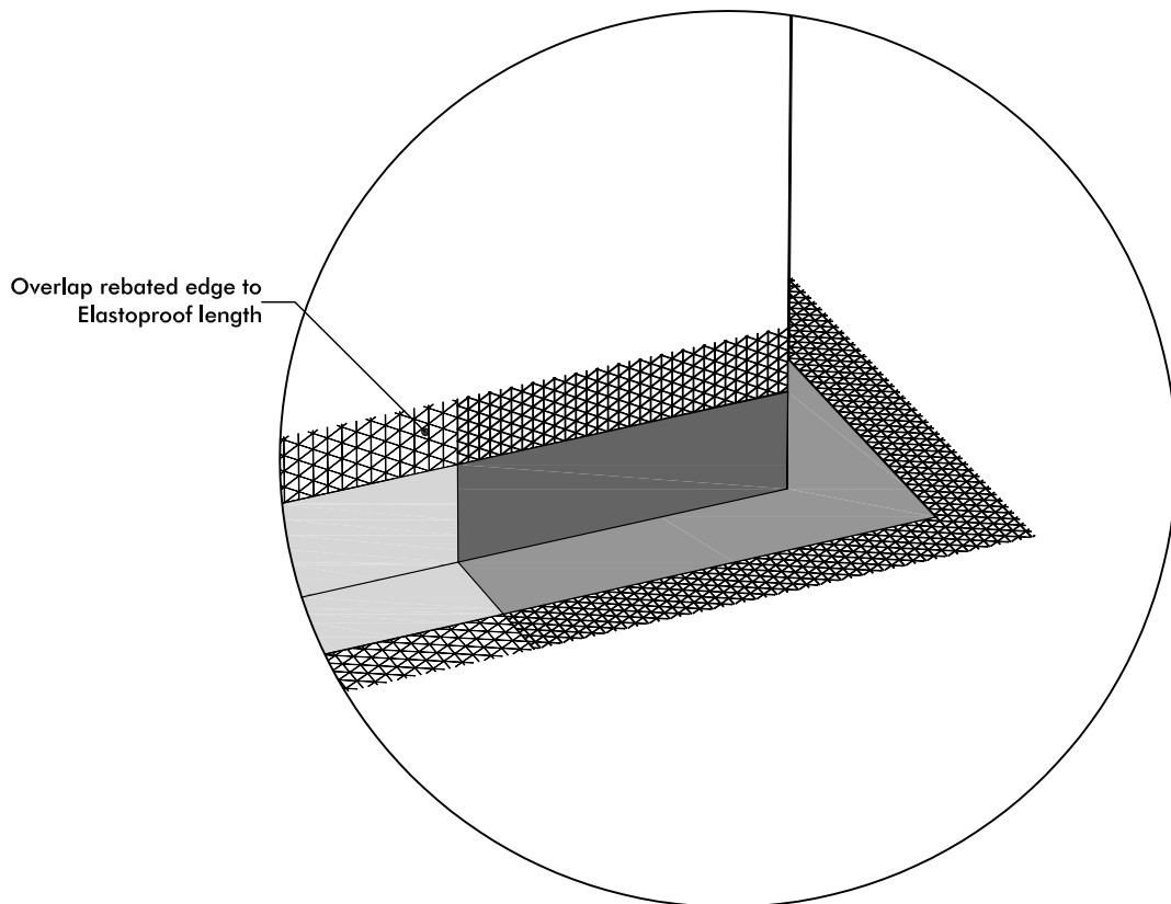
270° EXTERNAL CORNER
